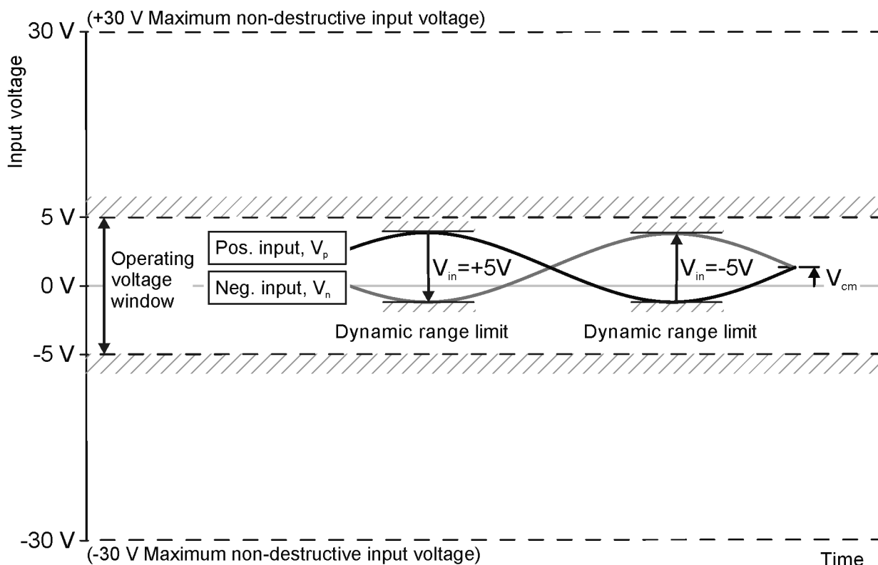
Fig. 4-2: Operating voltage window
