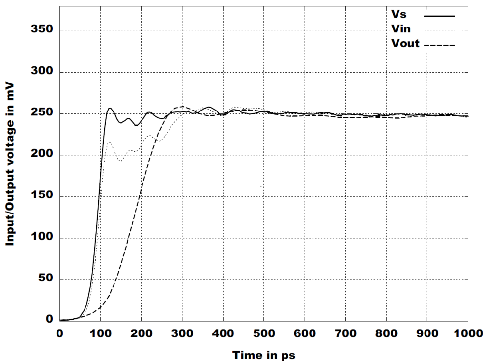
Fig. 5-8: Unloaded and loaded input signal and step response using the example of RT-ZS30
