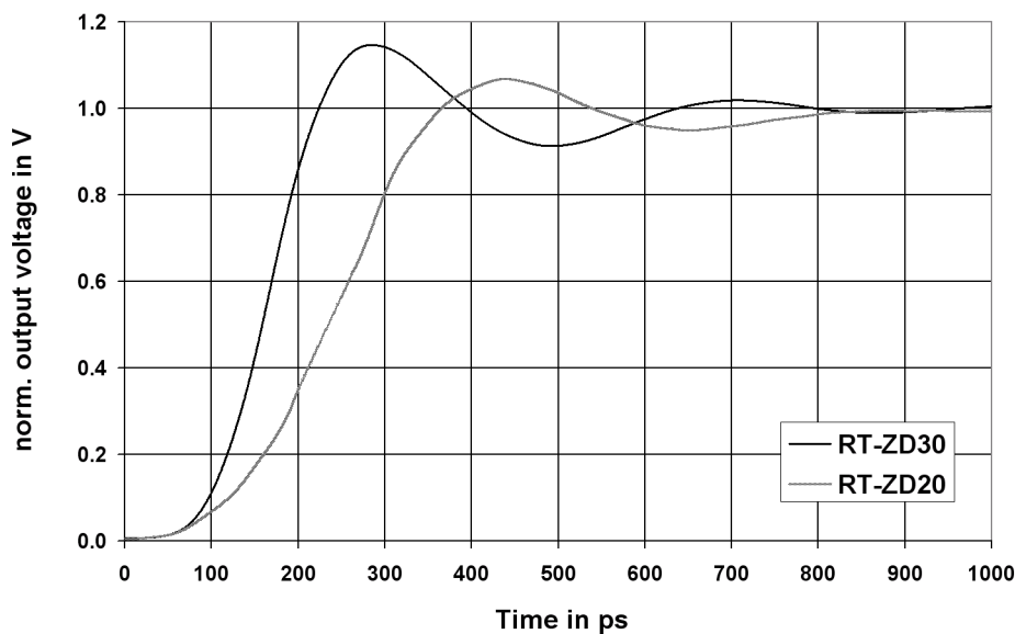
Fig. 5-3: Step response of the R&S RT-ZD20/30
