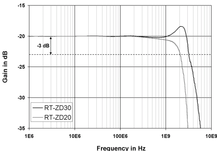
Fig. 5-2: Amplitude frequency response of the R&S RT-ZD20/30
