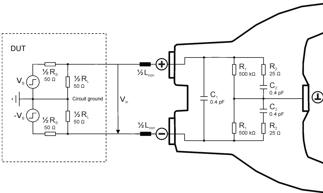
Fig. 5-1: Equivalent circuit model of the R&S RT-ZD20/30 probe
