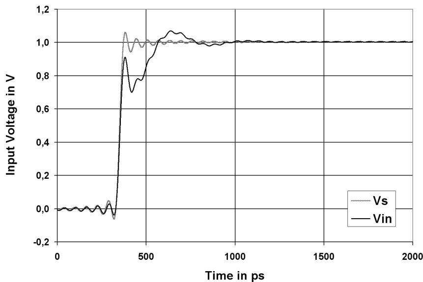
Fig. 5-7: Signal loading caused by the R&S RT-ZD20/30 probe
