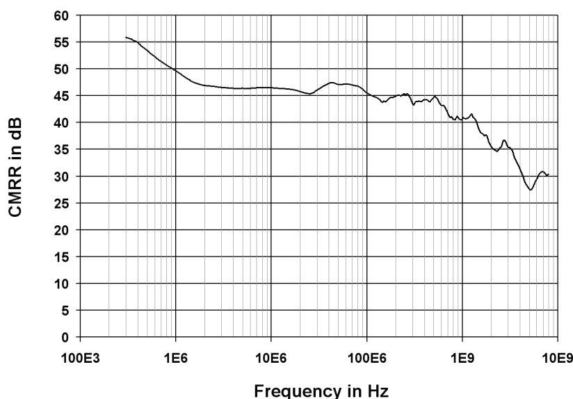
Fig. 5-5: Typical CMRR of the R&S RT-ZD20/30 probe as a function of frequency
