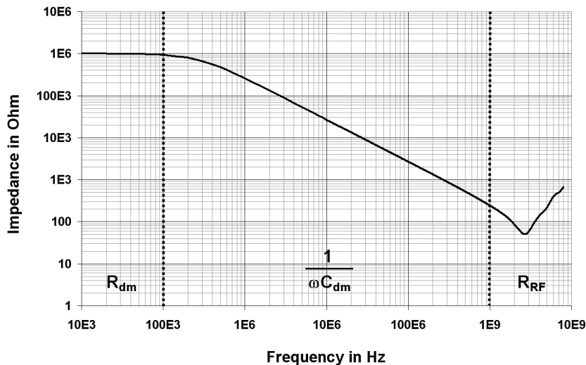
Fig. 5-6: Magnitude of the differential input impedance of the R&S RT-ZD20/30 probe as a function of frequency
