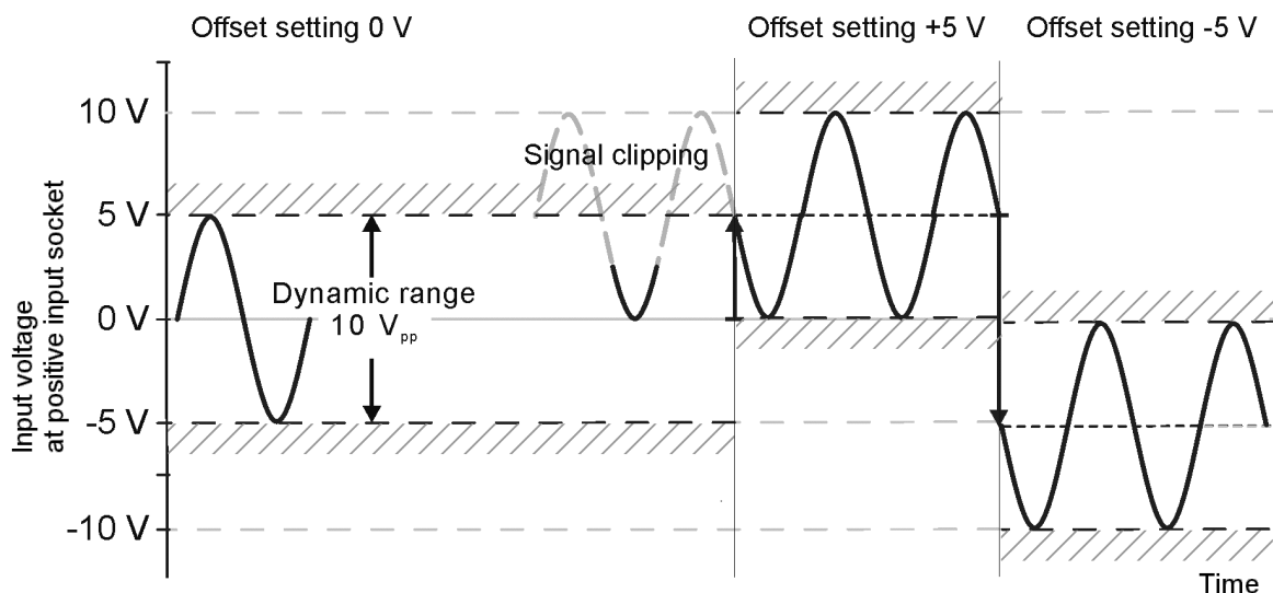
Fig. 2-2: Differential offset compensation voltage for single-ended measurement (negative signal socket connected to ground)
