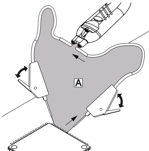
Fig. 5-4: Ground connection and connection inductance using the example of R&S RT-ZD20/30
